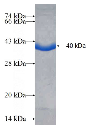
Recombinant Human SMG7 SDS-PAGE
