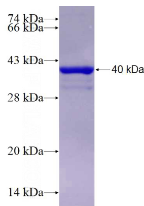
Recombinant Human KDM5B SDS-PAGE
