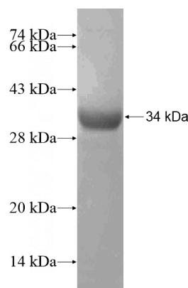
Recombinant Human Barkor SDS-PAGE
