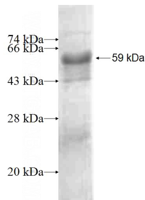
Recombinant Human PPP2R2C SDS-PAGE
