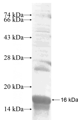
Recombinant Human PAX2 SDS-PAGE
