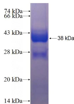
Recombinant Human IFRD2 SDS-PAGE
