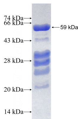
Recombinant Human NUP50 SDS-PAGE
