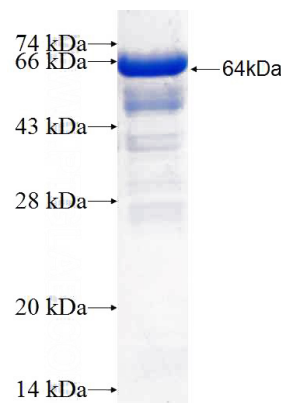
Recombinant Human PUM2 SDS-PAGE
