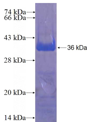
Recombinant Human ZNF394 SDS-PAGE
