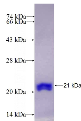
Recombinant Human UQCC SDS-PAGE
