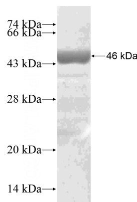
Recombinant Human CHMP4A SDS-PAGE
