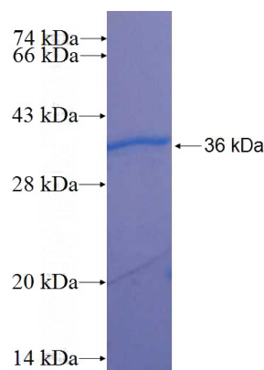
Recombinant Human FAM164B SDS-PAGE
