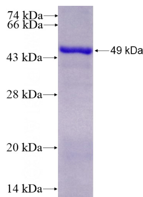
Recombinant Human STK11 SDS-PAGE
