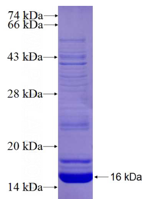
Recombinant Human RAB34 SDS-PAGE
