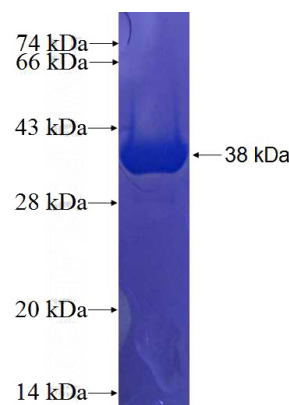
Recombinant Human CCDC102A SDS-PAGE
