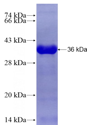
Recombinant Human ZC3H14 SDS-PAGE
