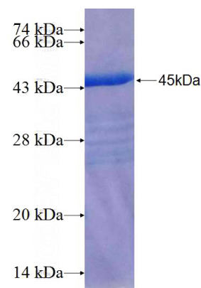
Recombinant Human STAMBPL1 SDS-PAGE
