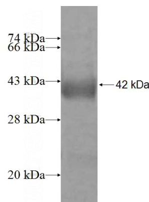
Recombinant Human FARS2 SDS-PAGE
