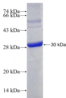
Recombinant Human SFMBT1 SDS-PAGE
