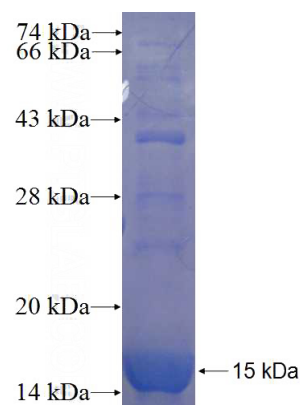
Recombinant Human KIF26A SDS-PAGE
