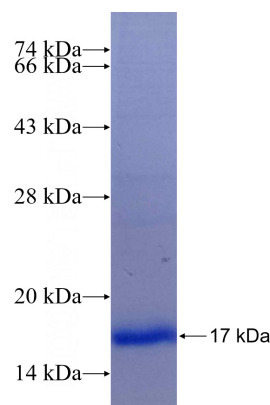
Recombinant Human ICMT SDS-PAGE
