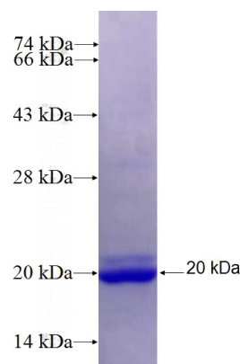
Recombinant Human ABCA7 SDS-PAGE
