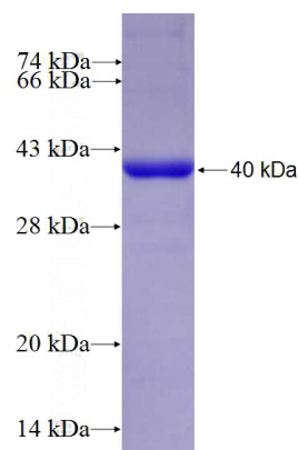
Recombinant Human LRRC49 SDS-PAGE
