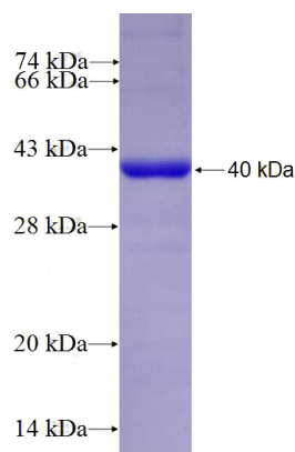
Recombinant Human LRRC49 SDS-PAGE
