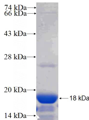
Recombinant Human ZFP30 SDS-PAGE
