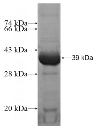
Recombinant Human C16orf89 SDS-PAGE
