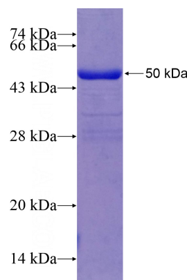
Recombinant Human PP2A SDS-PAGE
