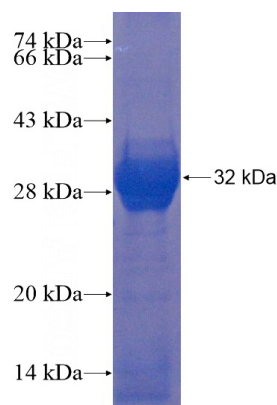
Recombinant Human GPR115 SDS-PAGE
