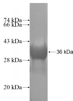
Recombinant Human FAM107B SDS-PAGE
