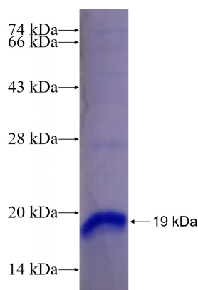
Recombinant Human ARHGEF7 SDS-PAGE
