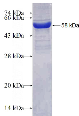
Recombinant Human METTL9 SDS-PAGE
