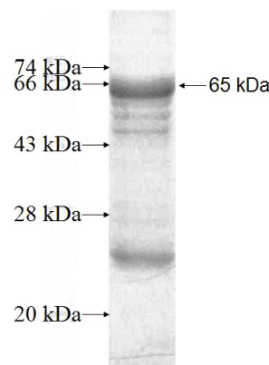
Recombinant Human LRP3 SDS-PAGE
