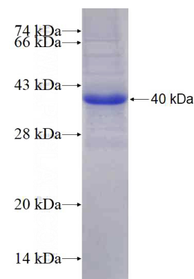
Recombinant Human ALG2 SDS-PAGE
