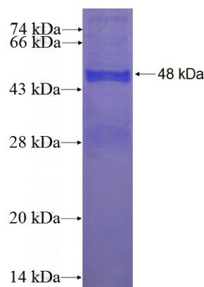
Recombinant Human FAHD1 SDS-PAGE
