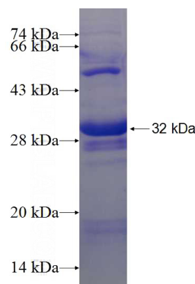
Recombinant Human IL-28RA SDS-PAGE
