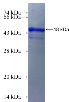
Recombinant Human CD48 SDS-PAGE
