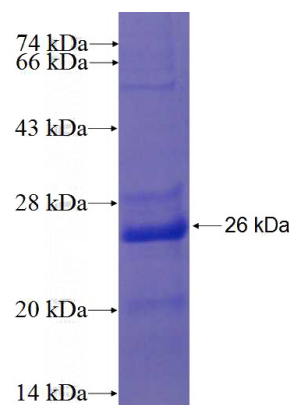
Recombinant Human RNASE9 SDS-PAGE
