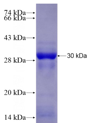
Recombinant Human ART1 SDS-PAGE
