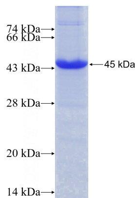
Recombinant Human PLA2R1 SDS-PAGE
