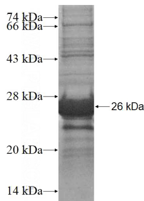
Recombinant Human KLHL4 SDS-PAGE
