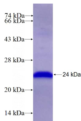
Recombinant Human ALKBH1 SDS-PAGE
