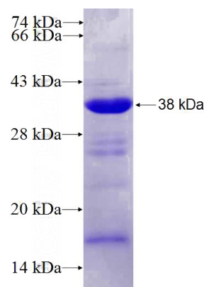
Recombinant Human ANGEL1 SDS-PAGE
