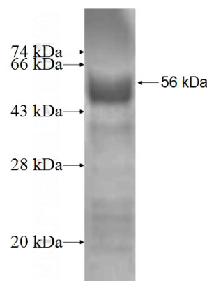
Recombinant Human FBXL18 SDS-PAGE
