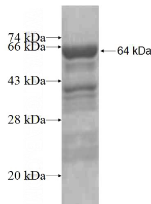
Recombinant Human CTNNA2 SDS-PAGE
