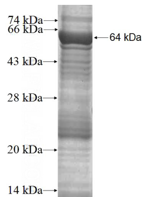
Recombinant Human FARP2 SDS-PAGE
