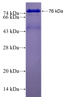
Recombinant Human TAF7 SDS-PAGE
