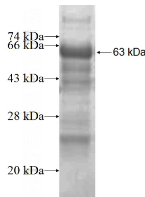
Recombinant Human TCF19 SDS-PAGE
