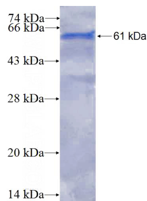
Recombinant Human SIAH2 SDS-PAGE
