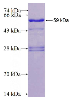
Recombinant Human CCND2 SDS-PAGE
