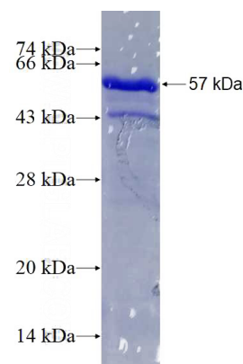
Recombinant Human USP29 SDS-PAGE
