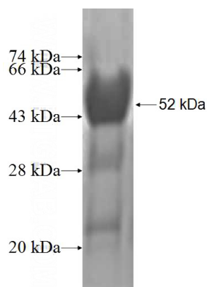
Recombinant Human PAFAH1B3 SDS-PAGE
